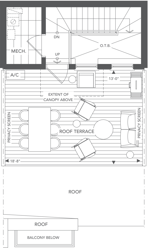
ROOFTOP TERRACE
