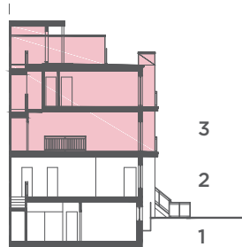
BLOCK 1 & 2 - TYP. SECTION
